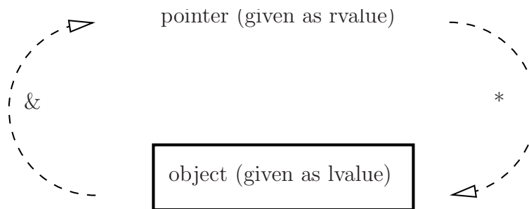
Figure 18: The address operator (left) and its inverse, the dereference operator (right)
