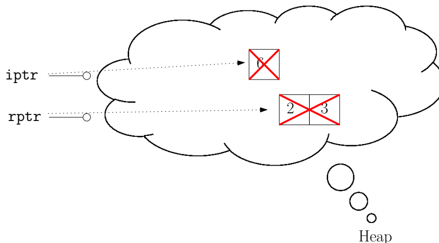
Figure 29: Safely deleting dynamically allocated objects: The two delete expressions involving iptr and rptr free the memory of the objects pointed to on the heap. Afterwards, the two pointers are set to 0 (visualized with —o ) in order to prevent accidental use of the expired object addresses.
