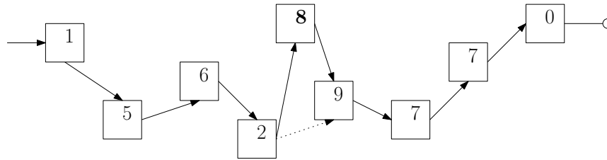
Figure 26: Inserting a new element (8) between two elements (2 and 9) of a list.
