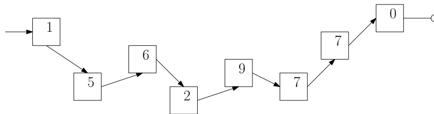
Figure 25: A list: a sequence of elements in which each element is pointing to the next one.
