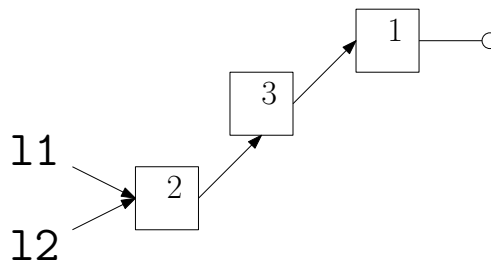
Figure 32: In the initialization list l2 = l1 , the head pointer of l2 is initialized with the head pointer of l1 , so that afterwards, l2 is not a copy of l1 but an alias.
