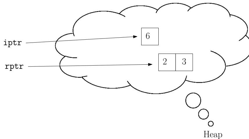
Figure 28: Dynamically allocating an integer and a rational number on the heap. The new expression returns the address of the newly allocated object; this address can be stored in a pointer variable through which the object can be accessed from now on.
