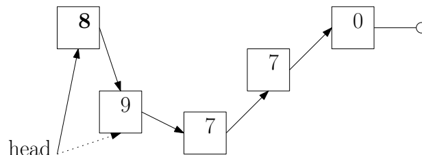
Figure 30: Inserting a new element (8) at the beginning of the list 9 \rightarrow 7 \rightarrow 7 \rightarrow 0 .
