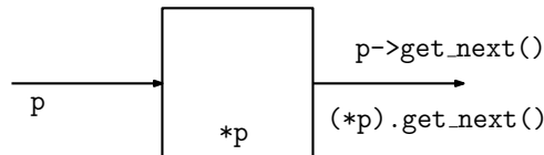
Figure 31: Setting p to p->get\_next() advances the pointer p (left arrow) to point to the next element (right arrow).
