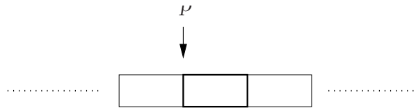
Figure 17: A pointer to T represents the address of an object of type T in the computer's main memory.
