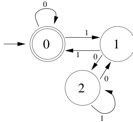
Figure 18: A deterministic finite automaton (DFA)
