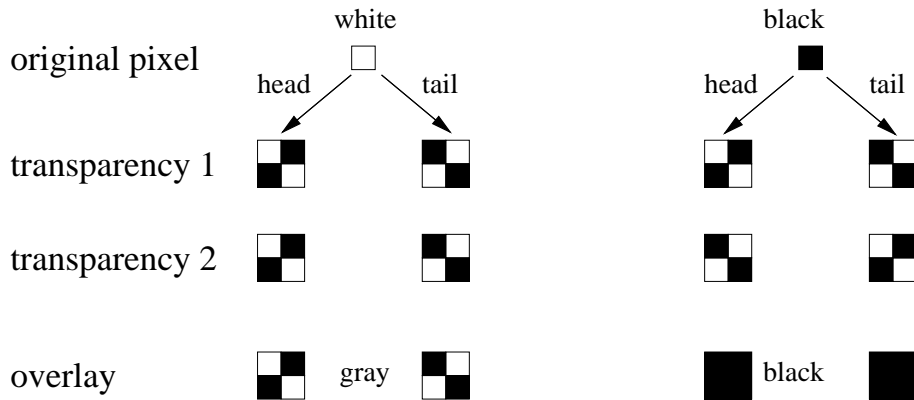
Figure 25: Visual cryptography: one pixel is split into two random “superpixels” of four pixels each, depending on the outcome of a fair coin flip
