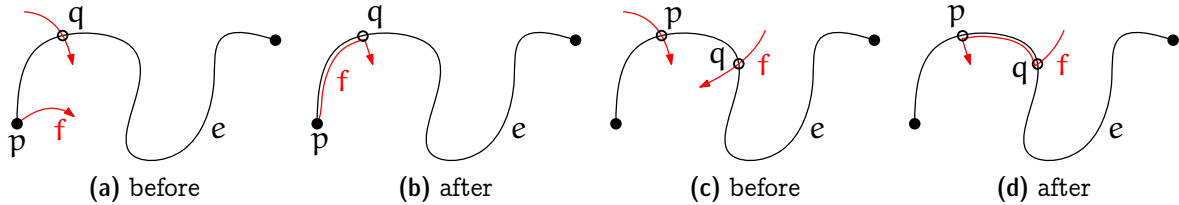
Figure 3.1: Redraw an edge f between two common points with another edge e to reduce the overall number of crossings. Figure (a) and (b) depict the situation where e and f are adjacent at p ; in this case the crossing at q can be eliminated. Figure (c) and (d) depict the situation where both p and q are crossings; in this case it depends on the local direction of f at these crossings: If f approaches e from the same side at p and q , then both crossings can be eliminated. Otherwise, as depicted here, a crossing at q remains.
