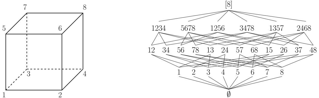
Figure 9.7: The cube (left) and its face lattice (right). Faces are named with the labels of their vertices.
