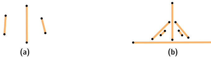
Figure 10.7: Sets of disjoint line segments that do not allow certain polygons.
