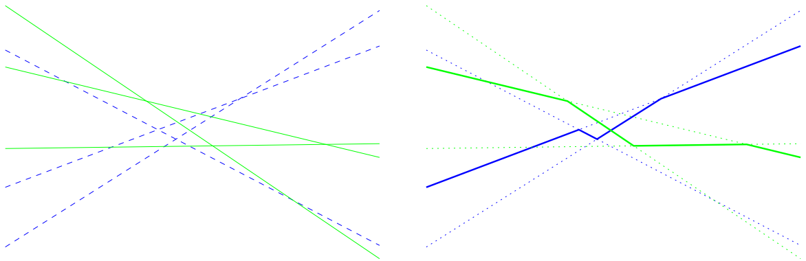
Figure 10.11: An arrangement of 3 green lines (solid) and 3 blue lines (dashed) and their median levels (marked bold on the right hand side).
