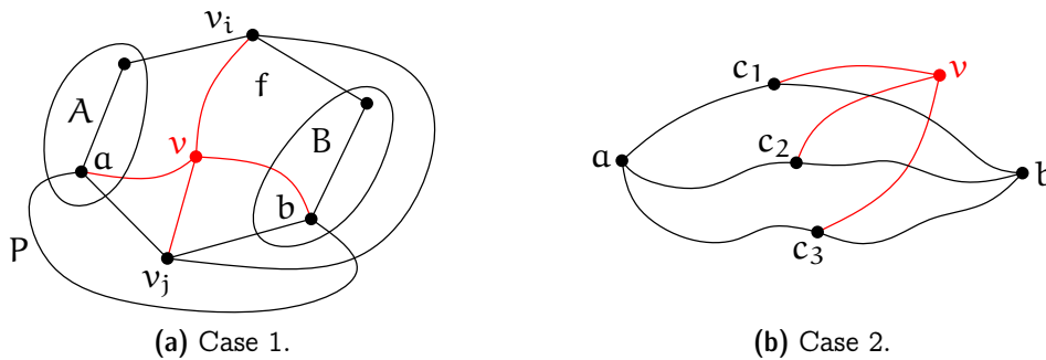
Figure 2.15: Illustration of the two cases in Theorem 2.25.
